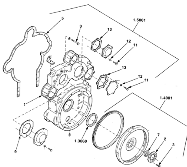
Flywheel Housing
