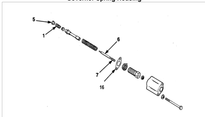
Governor Spring Housing
