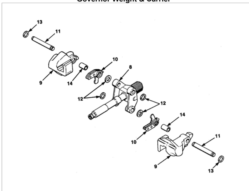
Governor Weight & Carrier
