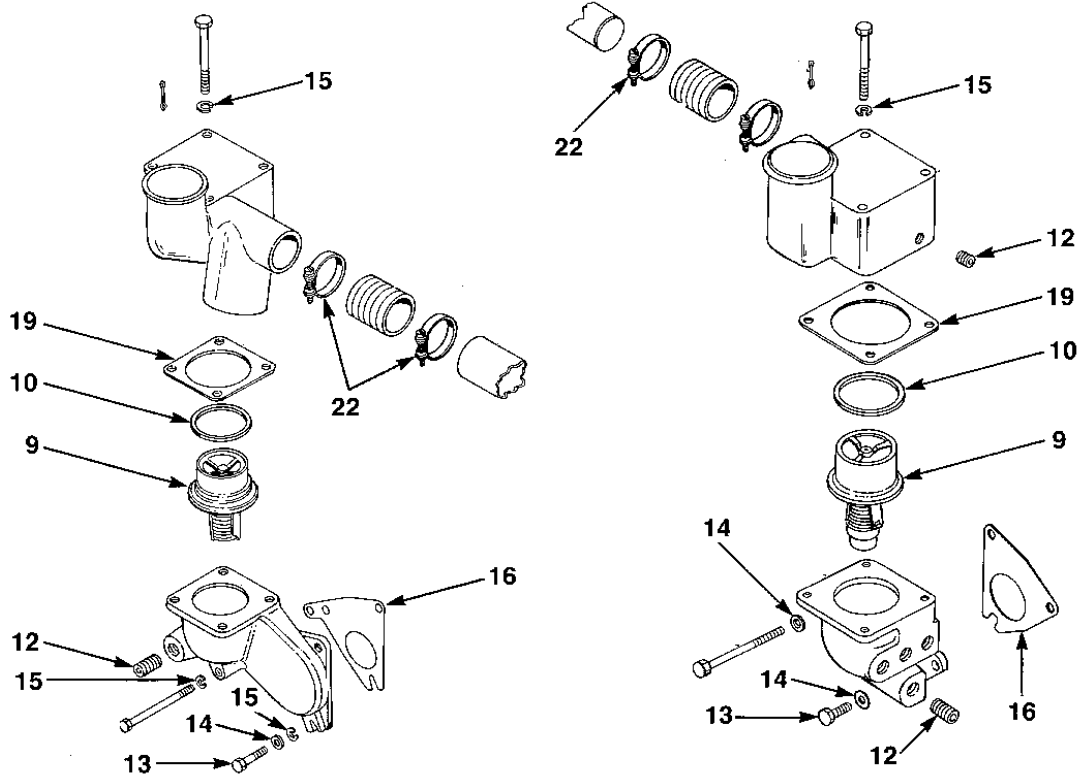
Thermostat
